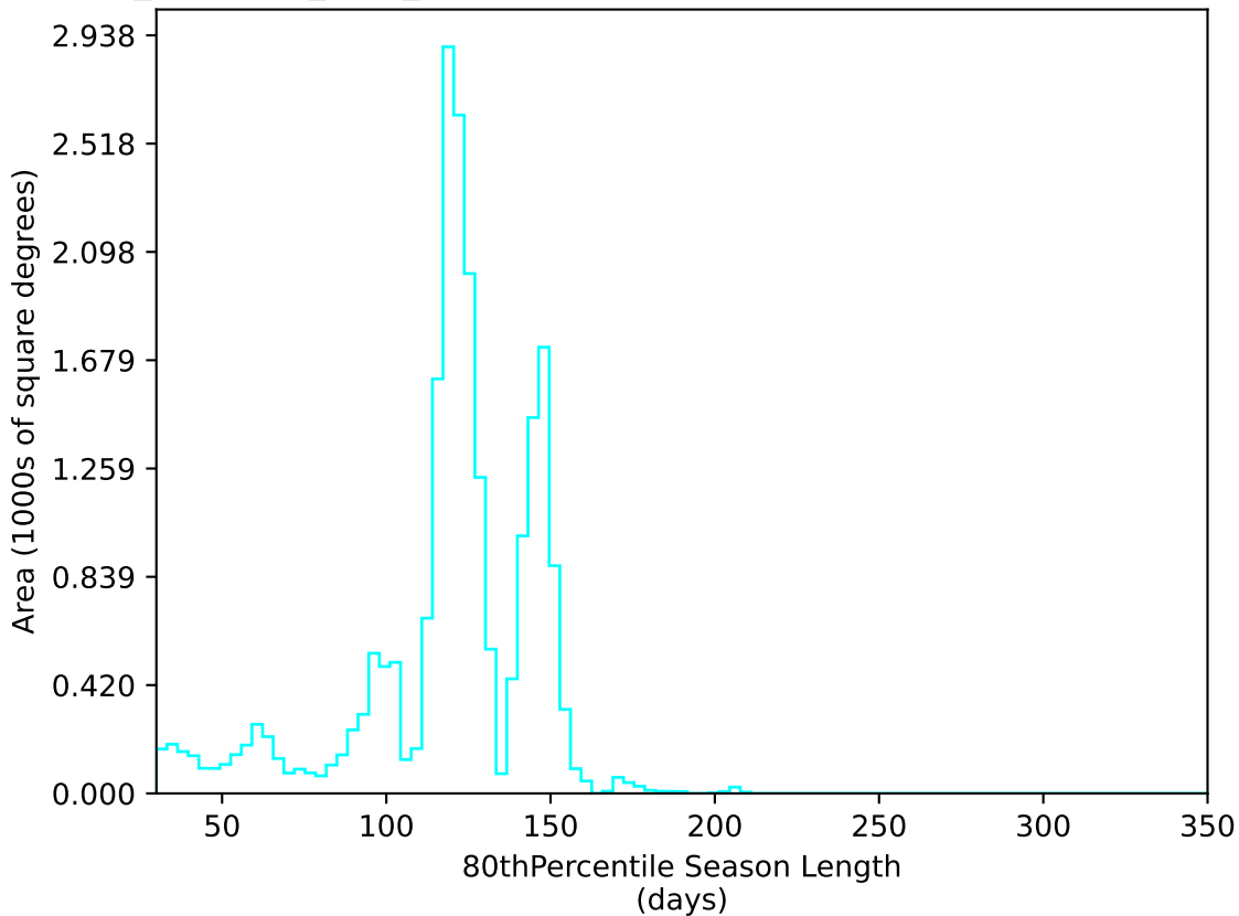
noroll_mjdp120_v3.4_10yrs All sky u band: 80thPercentile Season Length
