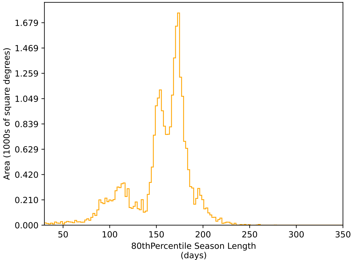
noroll_mjdp120_v3.4_10yrs All sky r band: 80thPercentile Season Length
