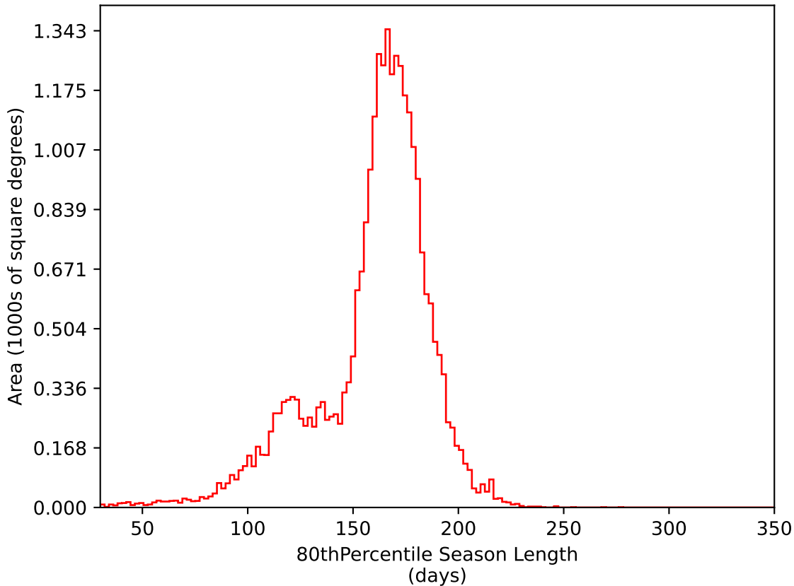
noroll_mjdp120_v3.4_10yrs All sky i band: 80thPercentile Season Length
