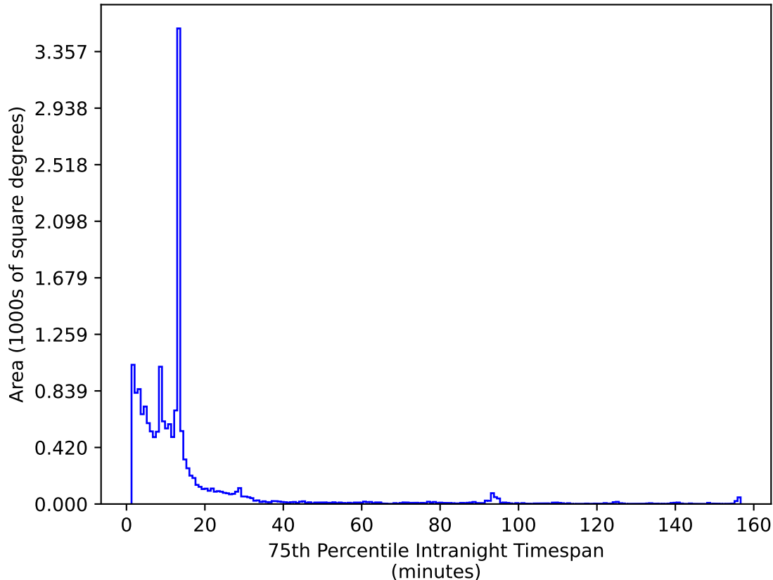
noroll_mjdp120_v3.4_10yrs WFD z band: 75th Percentile Intranight Timespan
