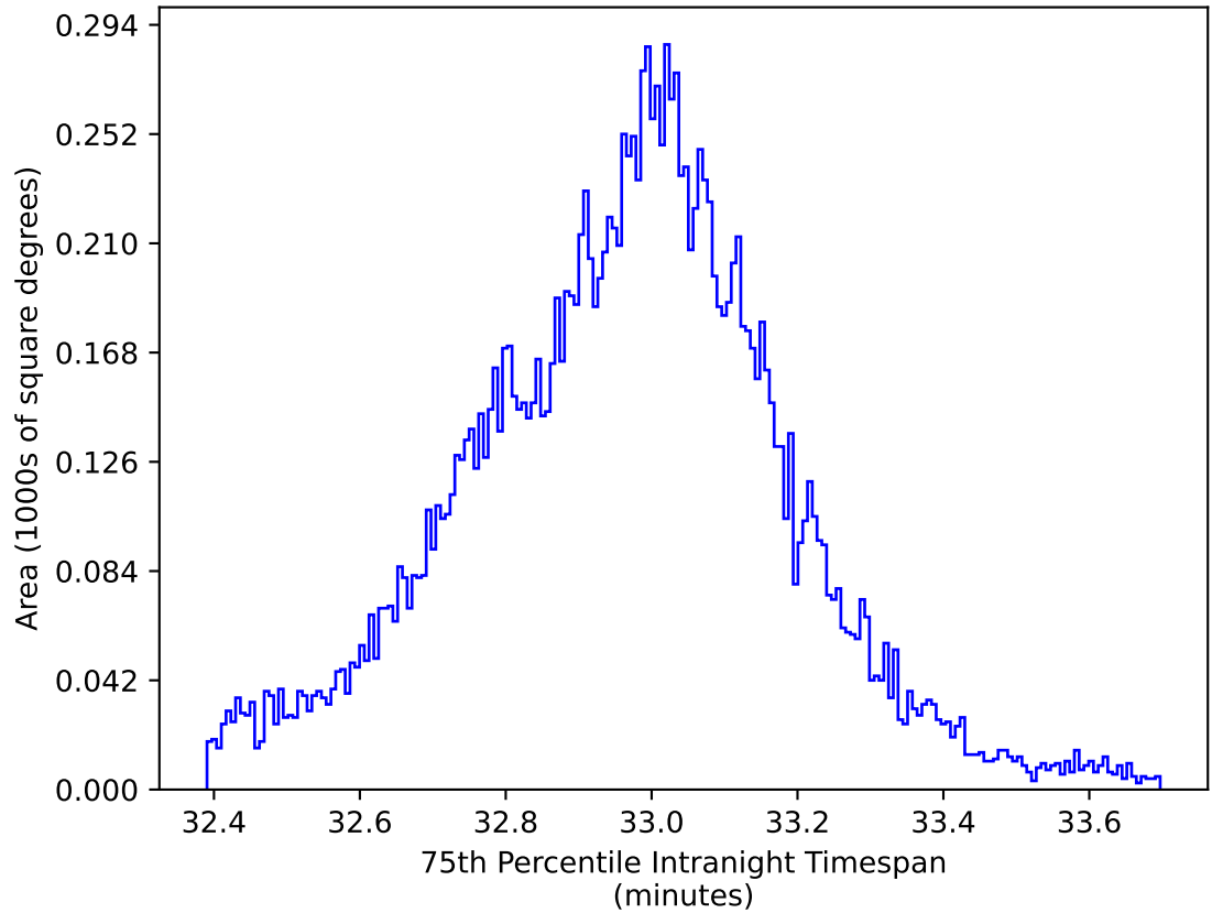
noroll_mjdp120_v3.4_10yrs WFD y band: 75th Percentile Intranight Timespan
