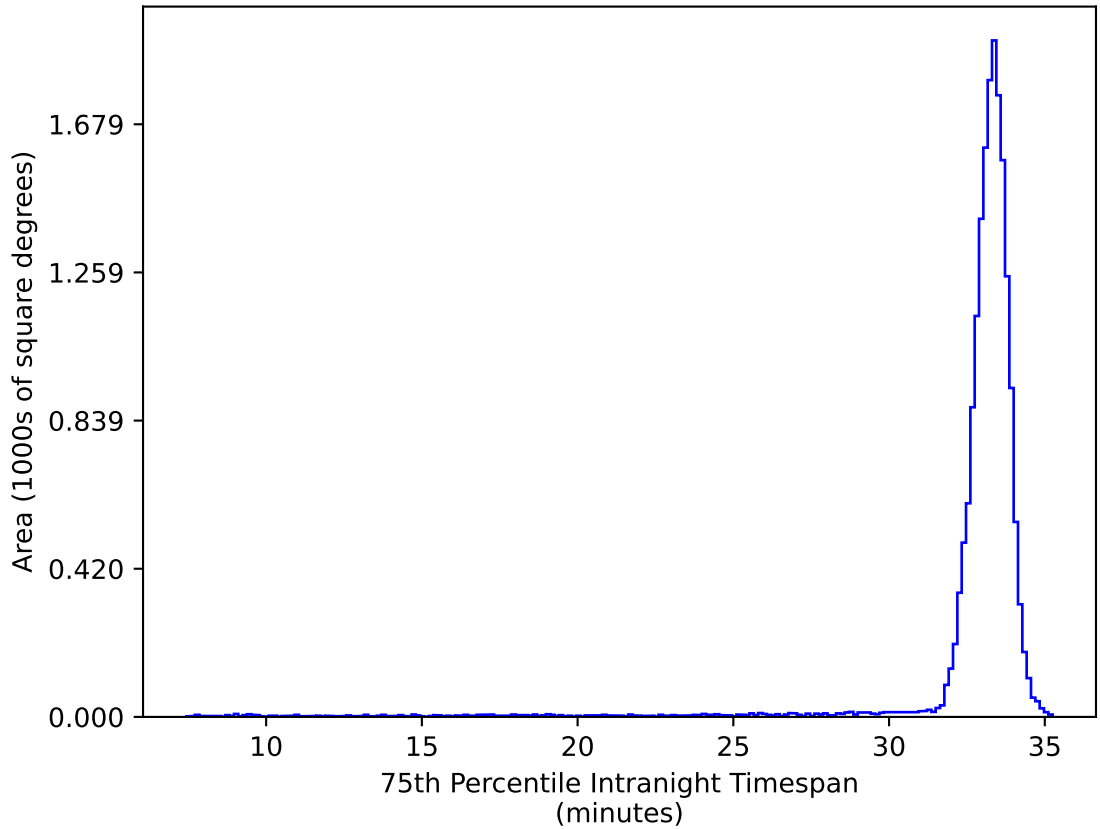
noroll_mjdp120_v3.4_10yrs WFD ug bands: 75th Percentile Intranight Timespan
