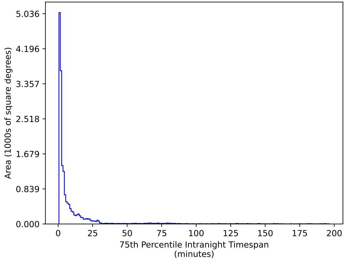
noroll_mjdp120_v3.4_10yrs WFD u band: 75th Percentile Intranight Timespan
