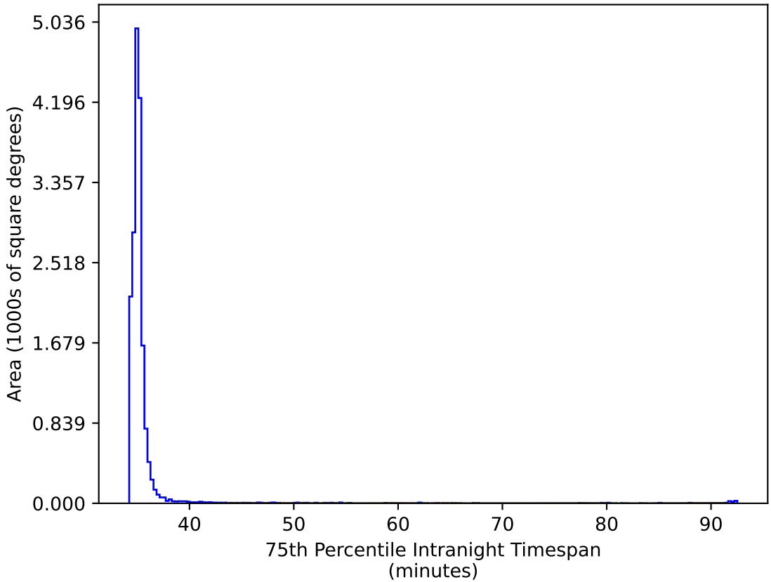
noroll_mjdp120_v3.4_10yrs WFD ri bands: 75th Percentile Intranight Timespan
