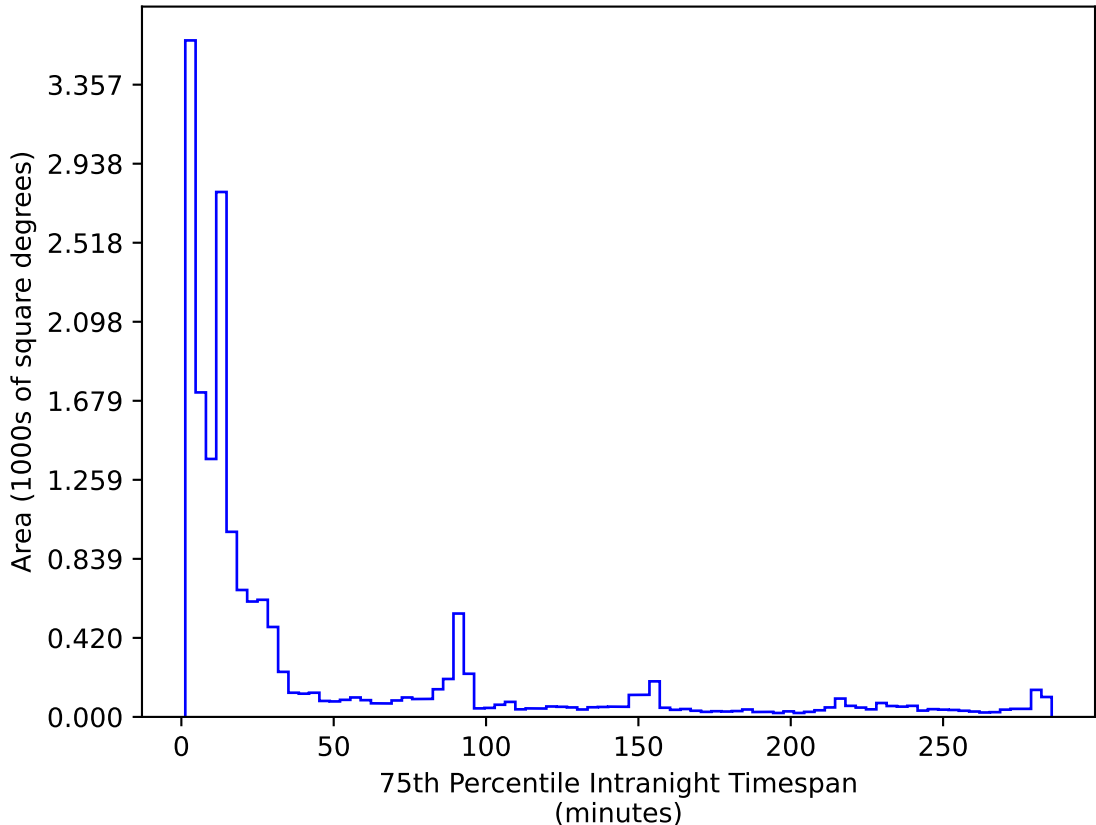
noroll_mjdp120_v3.4_10yrs WFD r band: 75th Percentile Intranight Timespan
