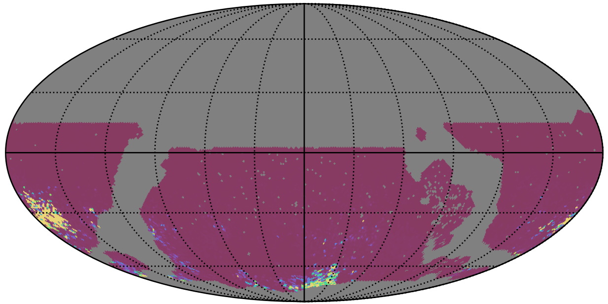
noroll_mjdp120_v3.4_10yrs WFD gr bands: 75th Percentile Intranight Timespan
