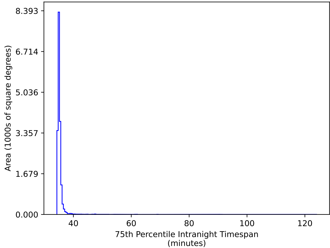
noroll_mjdp120_v3.4_10yrs WFD gr bands: 75th Percentile Intranight Timespan
