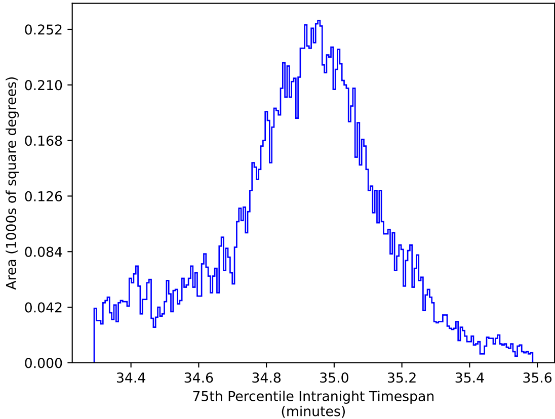
noroll_mjdp120_v3.4_10yrs WFD: 75th Percentile Intranight Timespan
