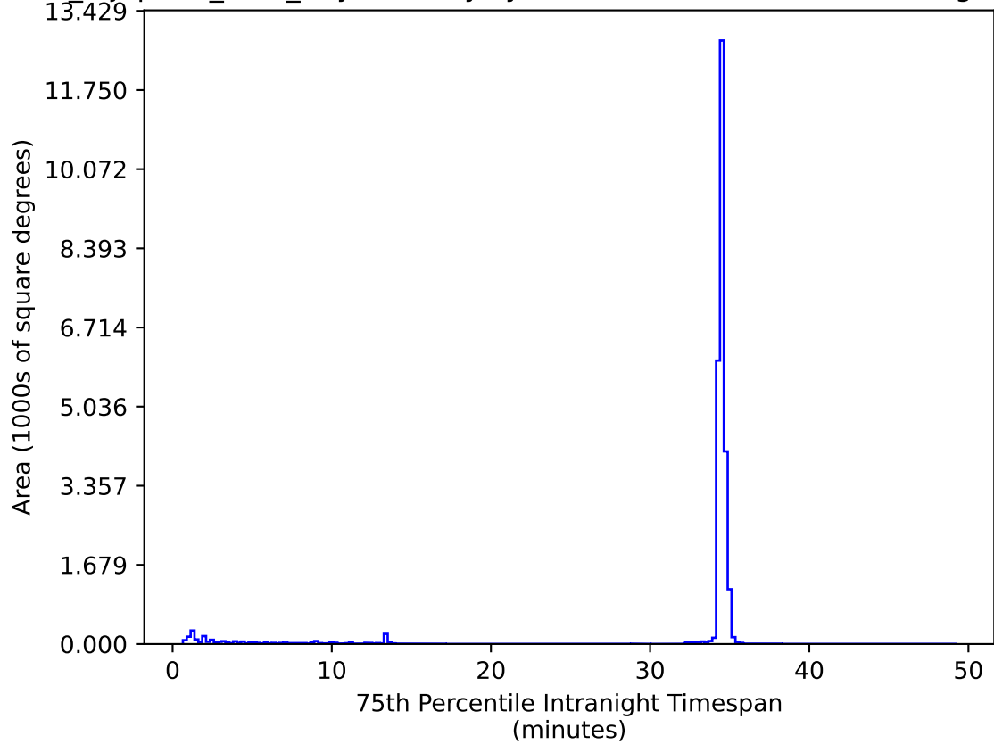
noroll_mjdp120_v3.4_10yrs All sky zy bands: 75th Percentile Intranight Timespan
