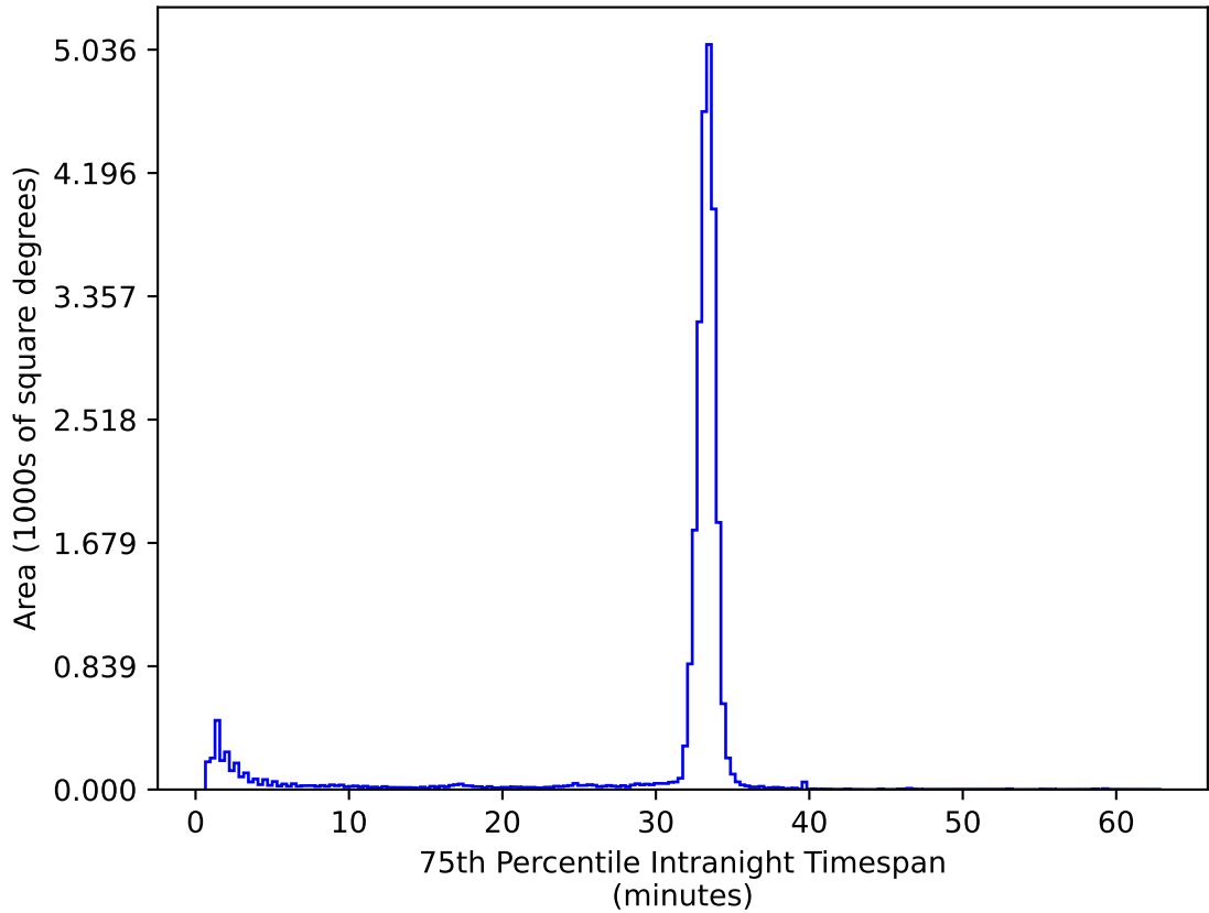
noroll_mjdp120_v3.4_10yrs All sky ug bands: 75th Percentile Intranight Timespan
