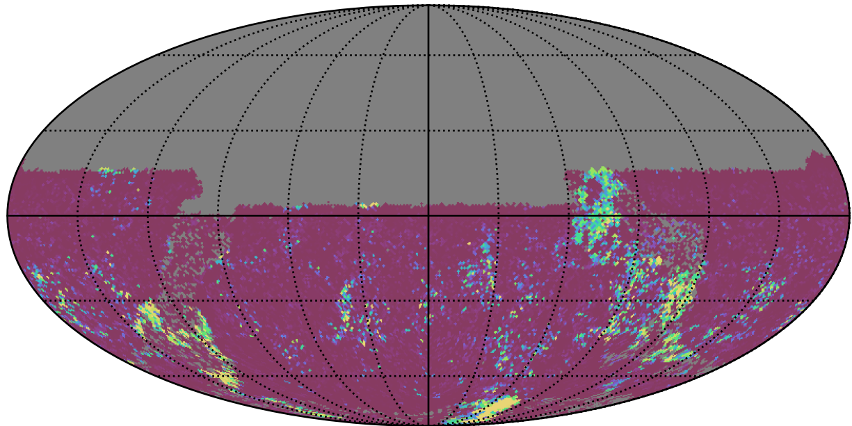
noroll_mjdp120_v3.4_10yrs All sky u band: 75th Percentile Intranight Timespan
