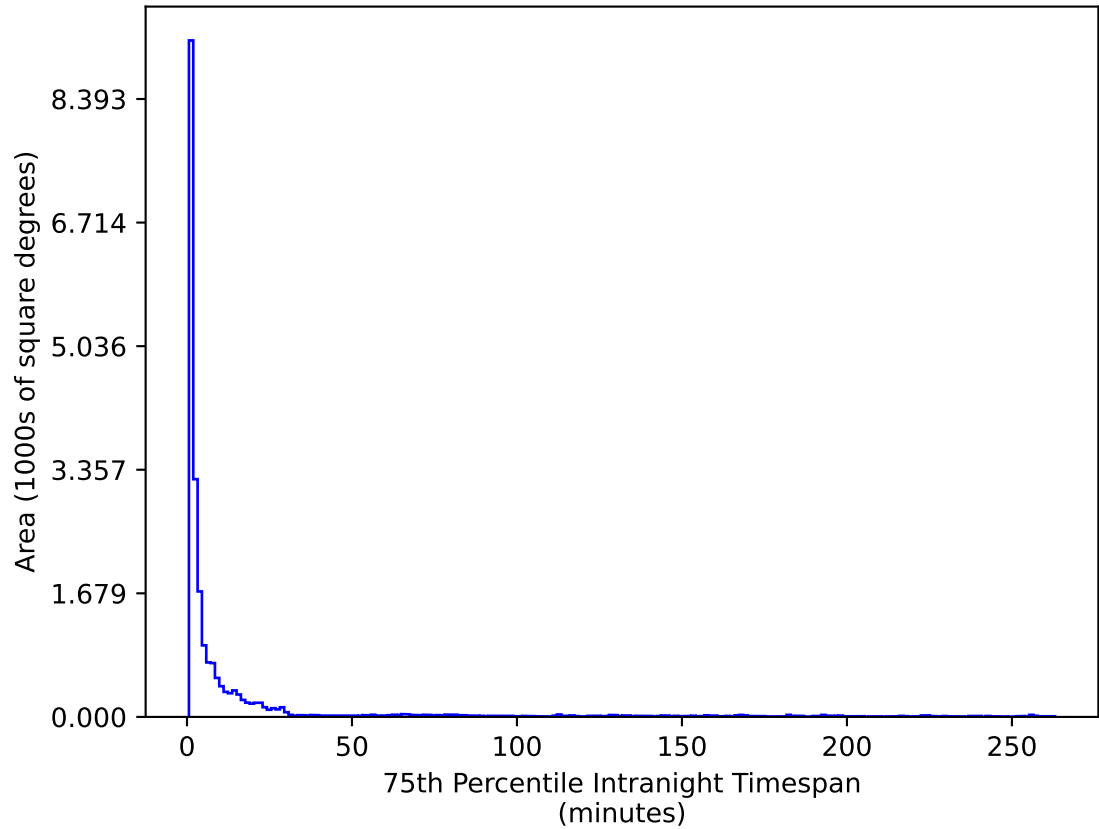
noroll_mjdp120_v3.4_10yrs All sky u band: 75th Percentile Intranight Timespan
