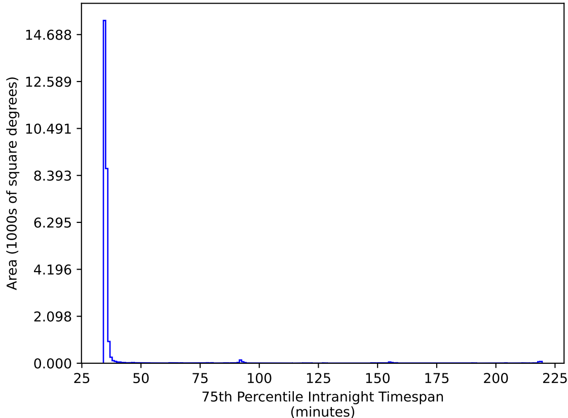
noroll_mjdp120_v3.4_10yrs All sky ri bands: 75th Percentile Intranight Timespan
