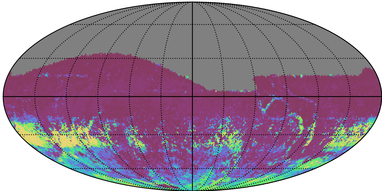
noroll_mjdp120_v3.4_10yrs All sky r band: 75th Percentile Intranight Timespan
