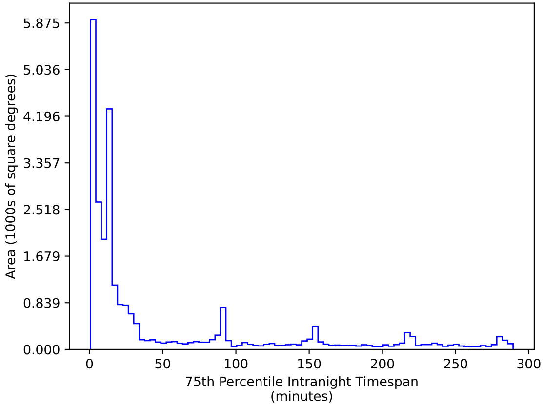
noroll_mjdp120_v3.4_10yrs All sky r band: 75th Percentile Intranight Timespan
