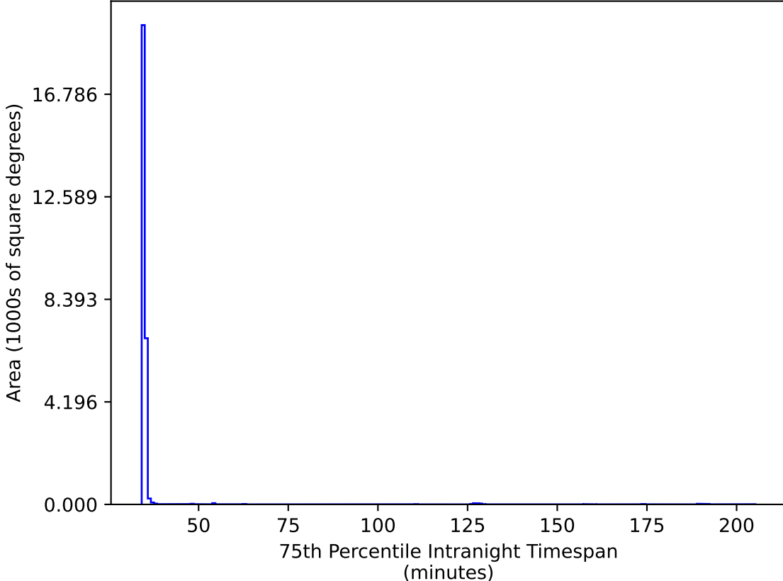
noroll_mjdp120_v3.4_10yrs All sky iz bands: 75th Percentile Intranight Timespan
