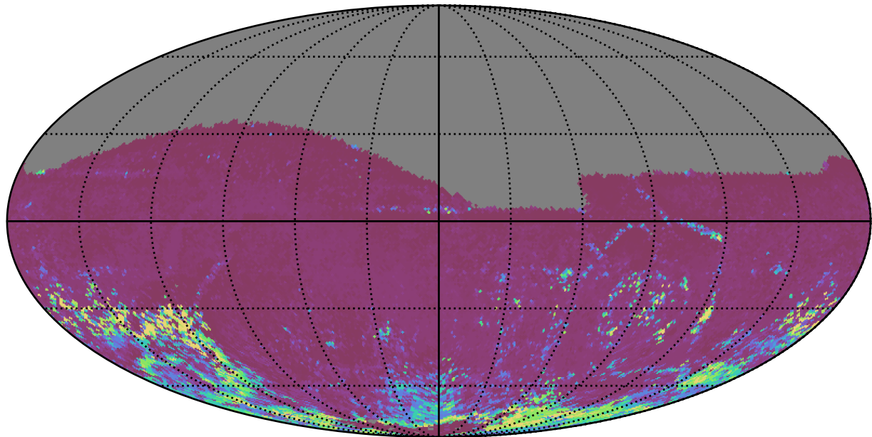
noroll_mjdp120_v3.4_10yrs All sky i band: 75th Percentile Intranight Timespan
