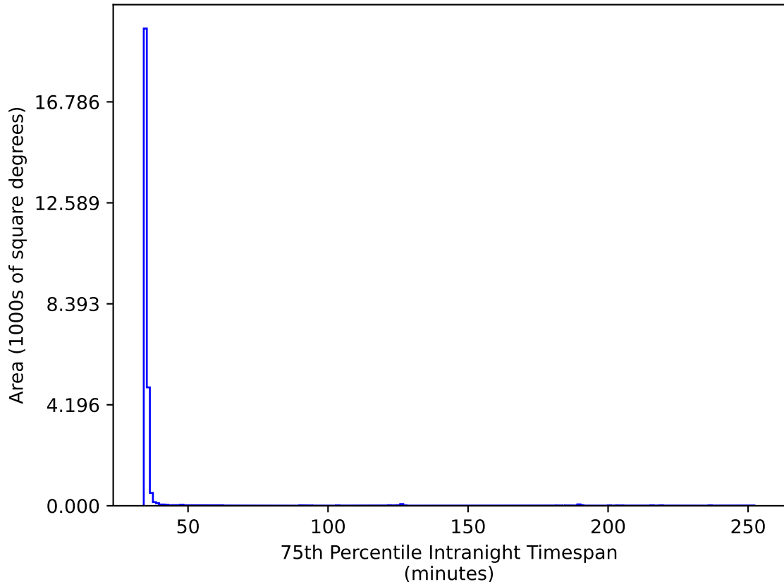
noroll_mjdp120_v3.4_10yrs All sky gr bands: 75th Percentile Intranight Timespan
