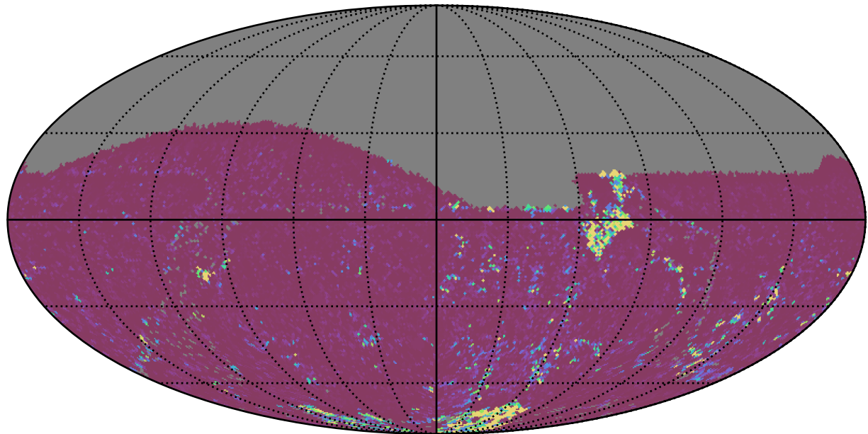
noroll_mjdp120_v3.4_10yrs All sky g band: 75th Percentile Intranight Timespan
