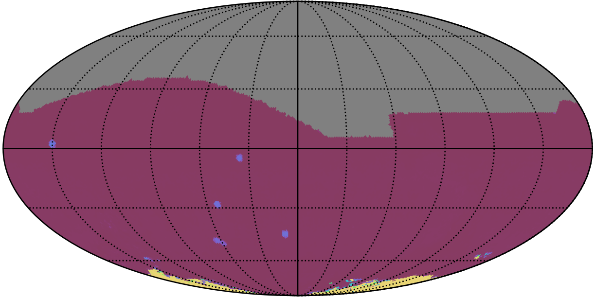
noroll_mjdp120_v3.4_10yrs All sky all bands: 75th Percentile Intranight Timespan
