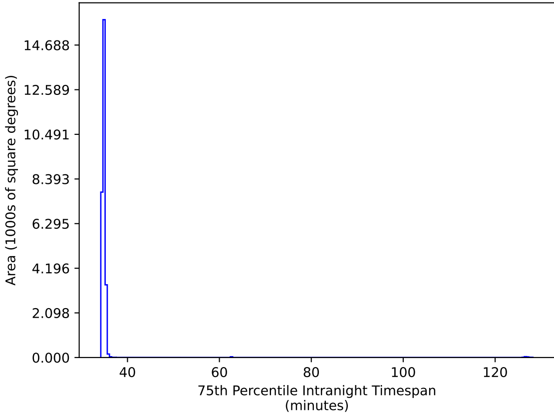
noroll_mjdp120_v3.4_10yrs All sky: 75th Percentile Intranight Timespan
