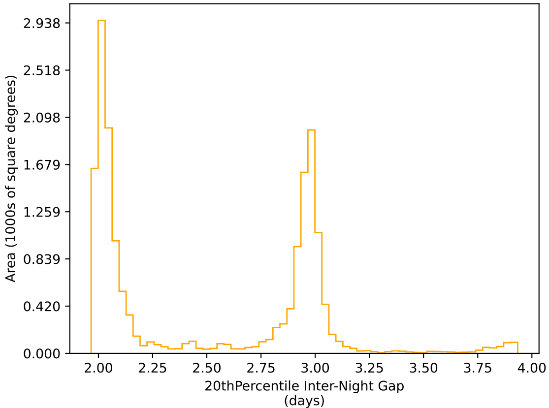
noroll_mjdp120_v3.4_10yrs WFD r band: 20thPercentile Inter-Night Gap
