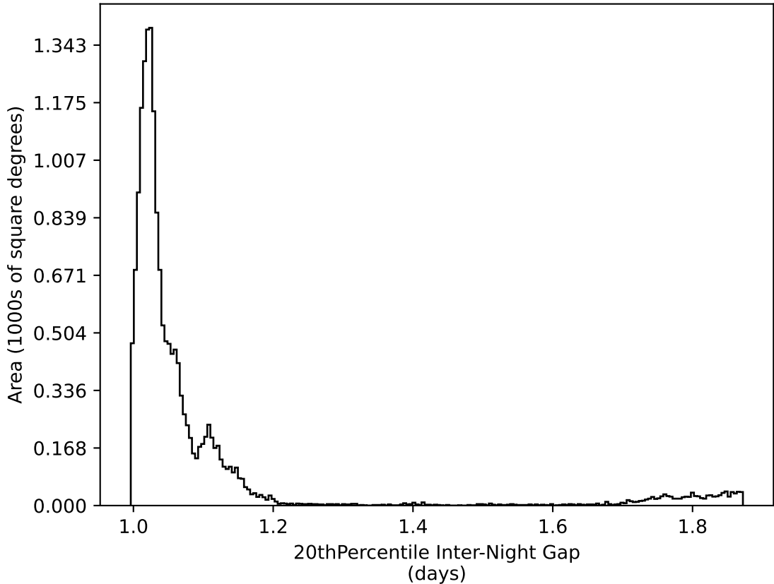
noroll_mjdp120_v3.4_10yrs WFD all bands: 20thPercentile Inter-Night Gap
