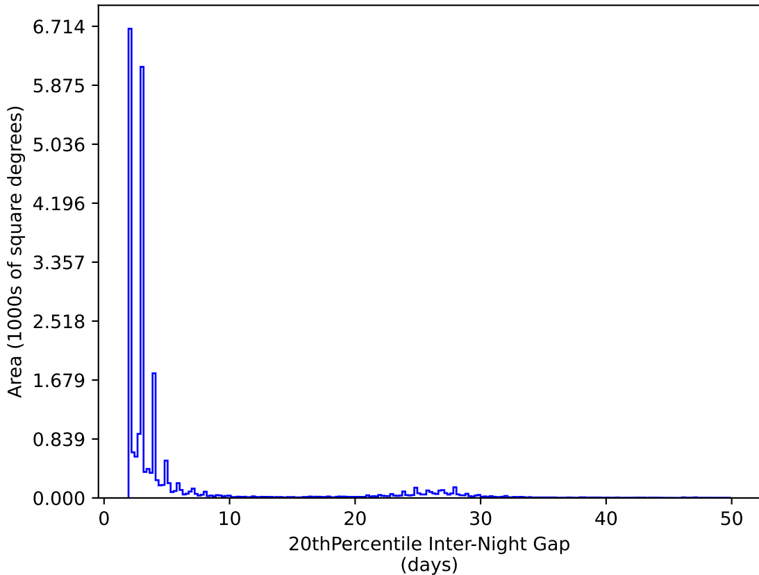
noroll_mjdp120_v3.4_10yrs All sky y band: 20thPercentile Inter-Night Gap
