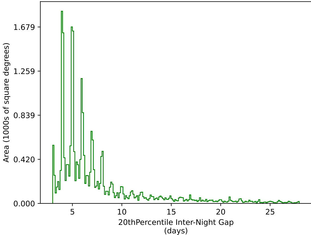
noroll_mjdp120_v3.4_10yrs All sky g band: 20thPercentile Inter-Night Gap
