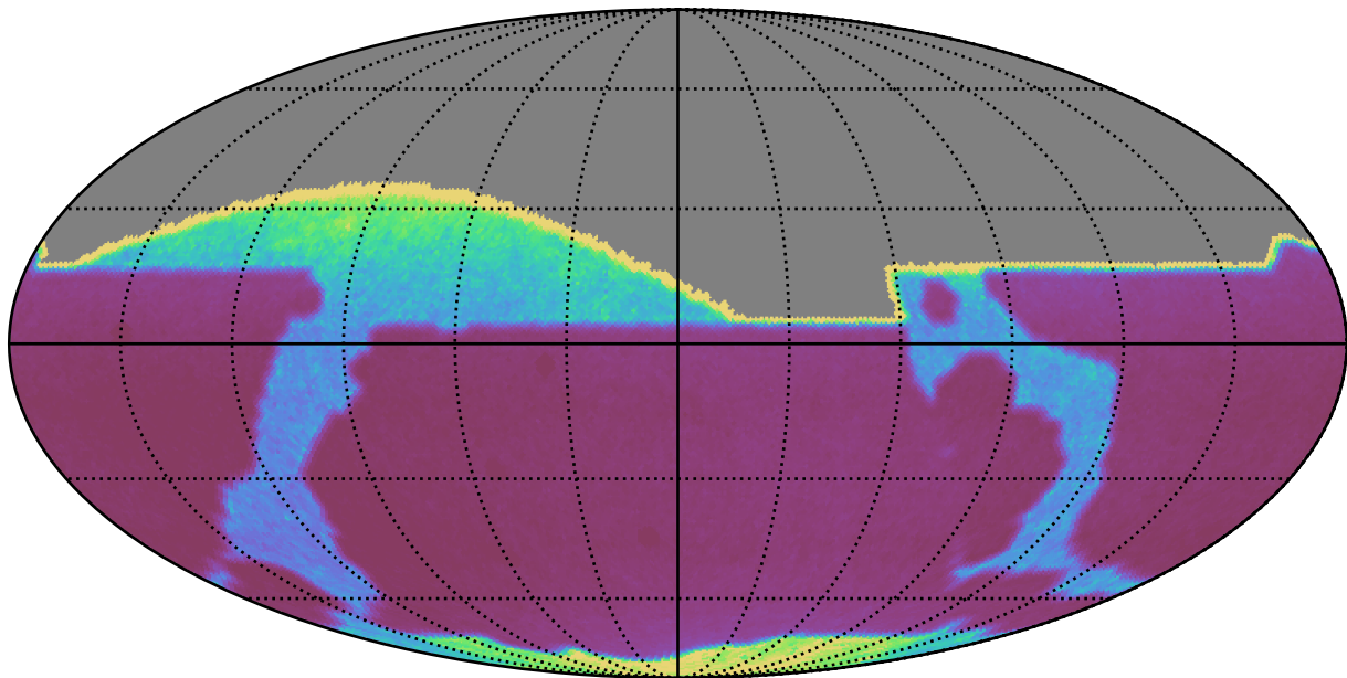
noroll_mjdp120_v3.4_10yrs : properMotion
