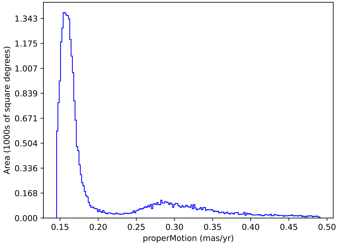
noroll_mjdp120_v3.4_10yrs : properMotion
