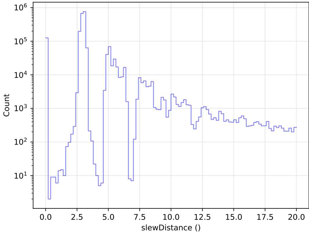
noroll_mjdp120_v3.4_10yrs All visits: Zoom Slew Distance Histogram
