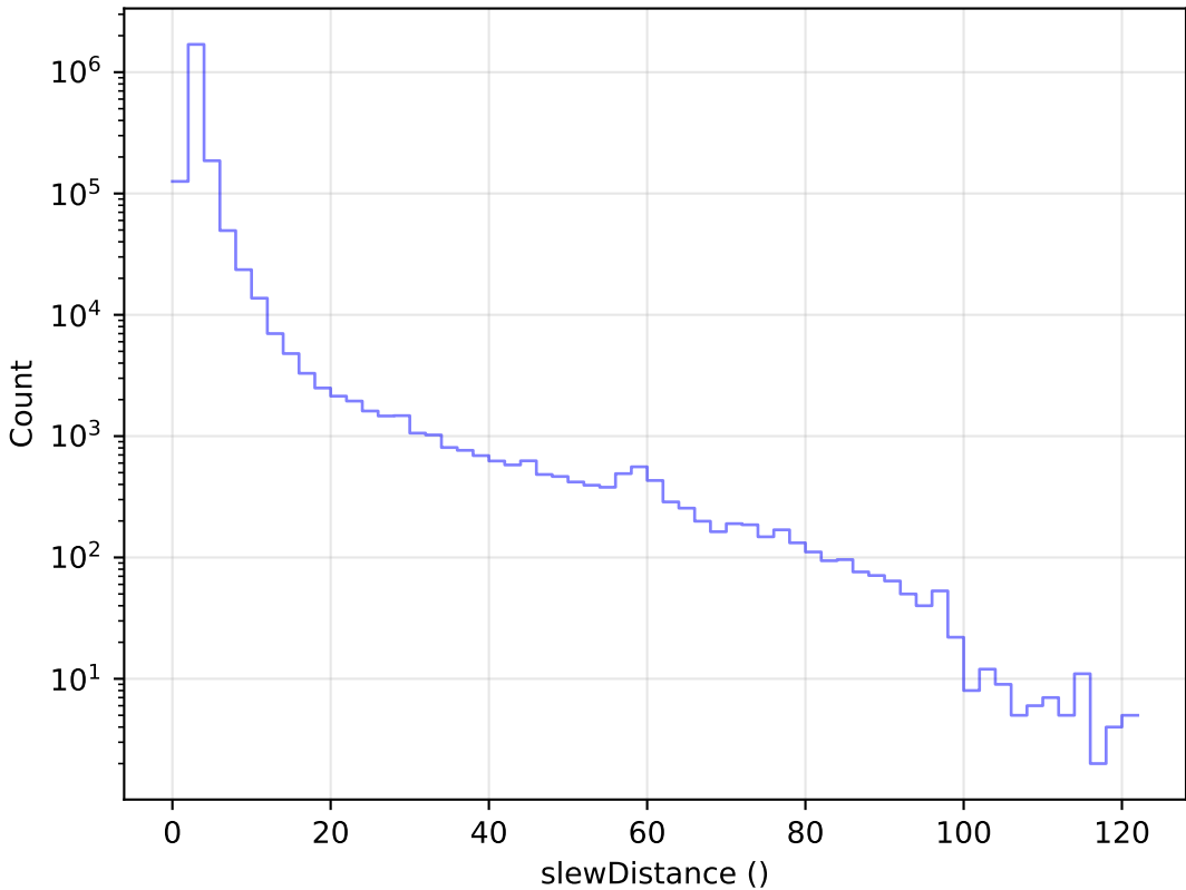
noroll_mjdp120_v3.4_10yrs All visits: Slew Distance Histogram
