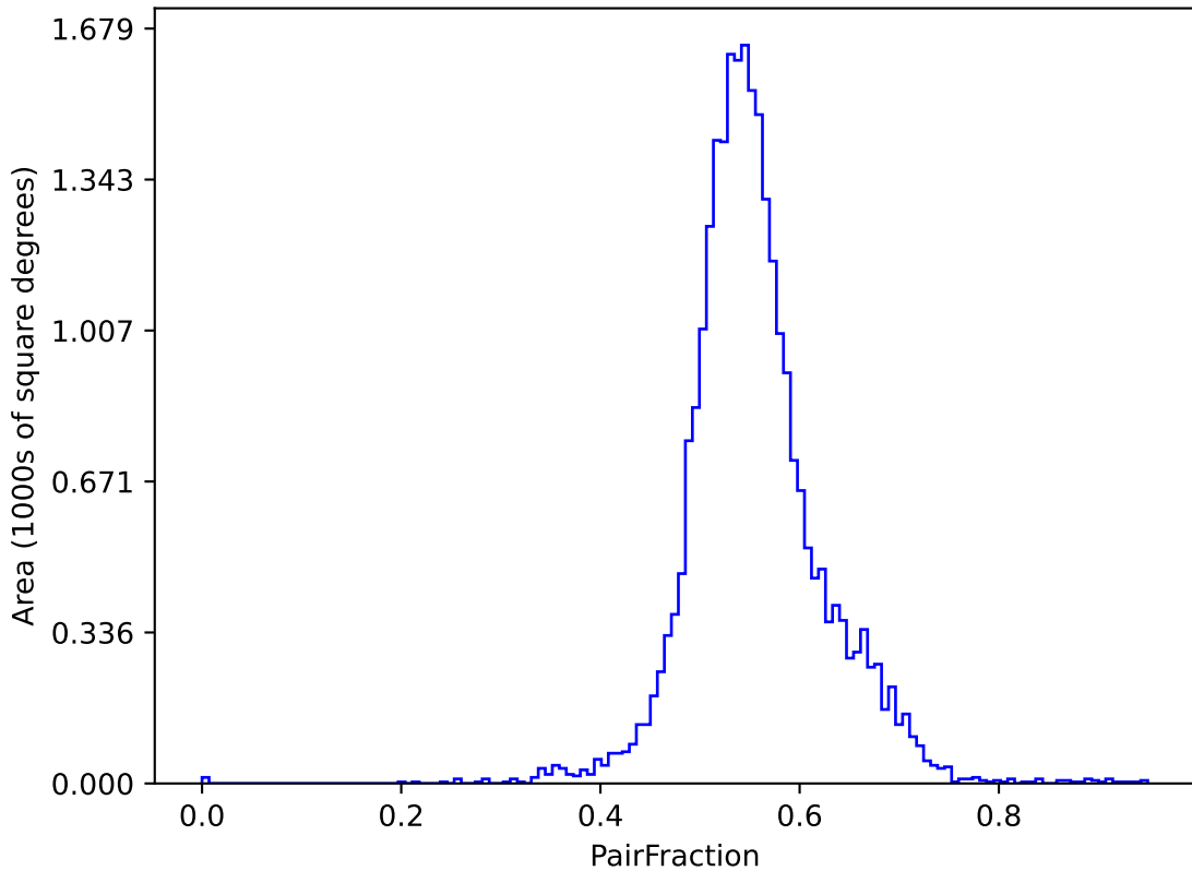
noroll_mjdp120_v3.4_10yrs (g or r or i): PairFraction
