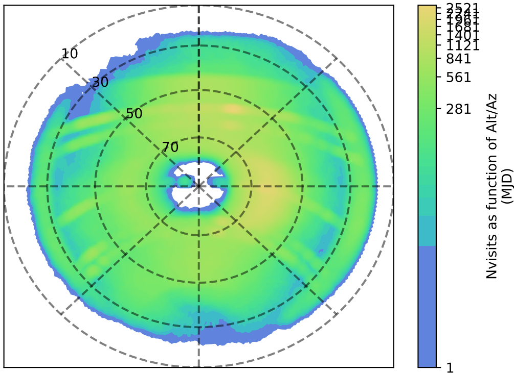
noroll_mjdp120_v3.4_10yrs z: Nvisits as function of Alt/Az
