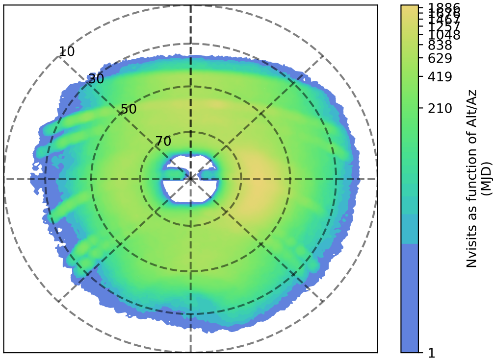
noroll_mjdp120_v3.4_10yrs y: Nvisits as function of Alt/Az
