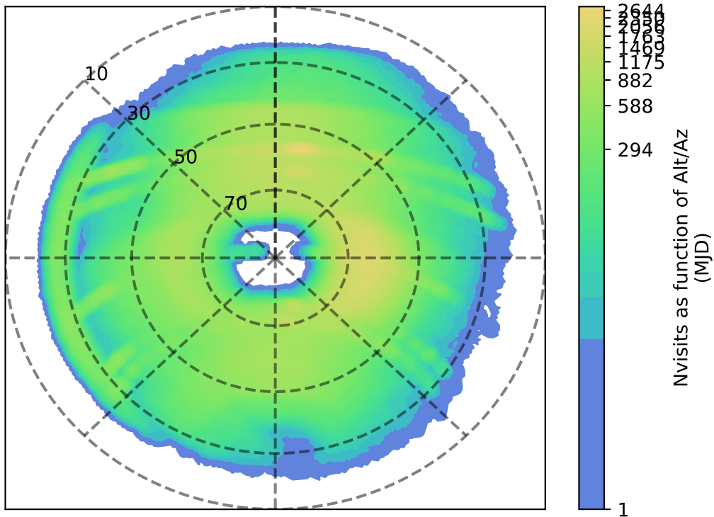
noroll_mjdp120_v3.4_10yrs r: Nvisits as function of Alt/Az
