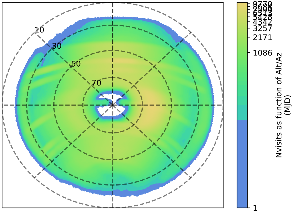
noroll_mjdp120_v3.4_10yrs : Nvisits as function of Alt/Az
