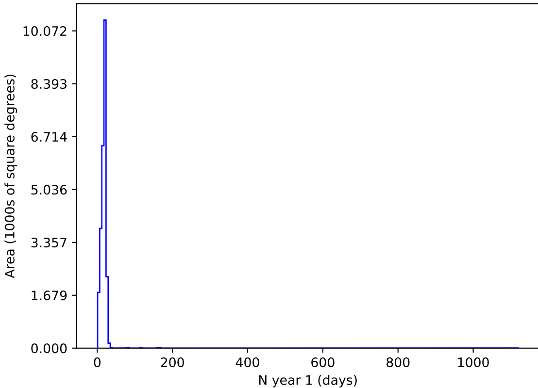
noroll_mjdp120_v3.4_10yrs y and night < 365: N year 1
