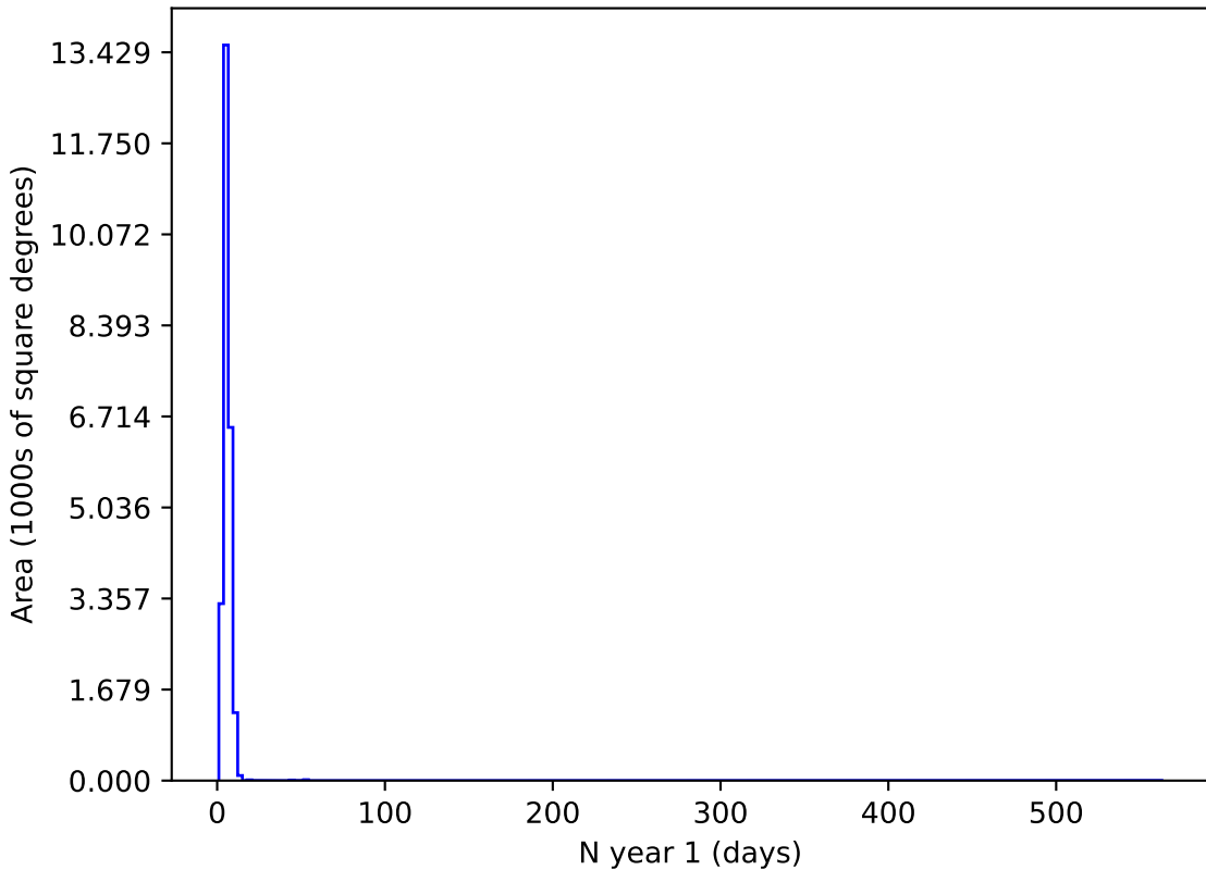
noroll_mjdp120_v3.4_10yrs u and night &lt; 365: N year 1
