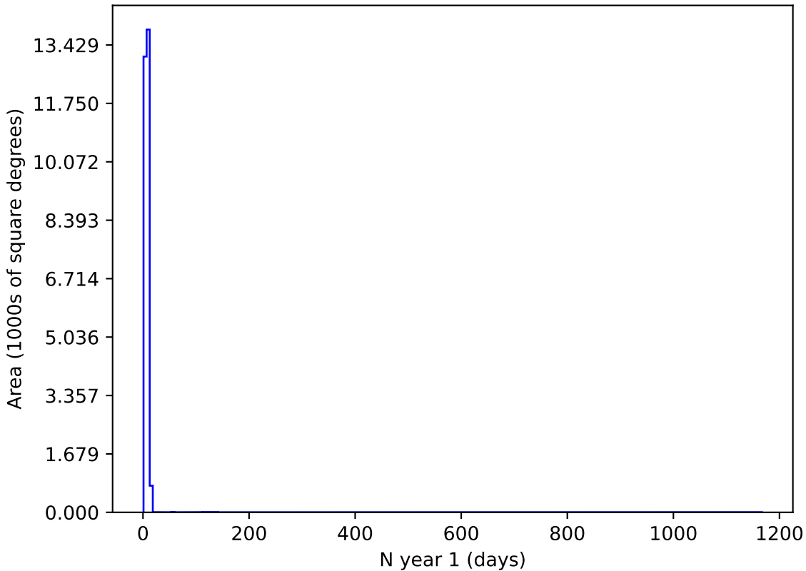
noroll_mjdp120_v3.4_10yrs g and night < 365: N year 1
