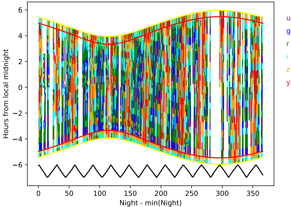
noroll_mjdp120_v3.4_10yrs year 9-10: Hourglass
