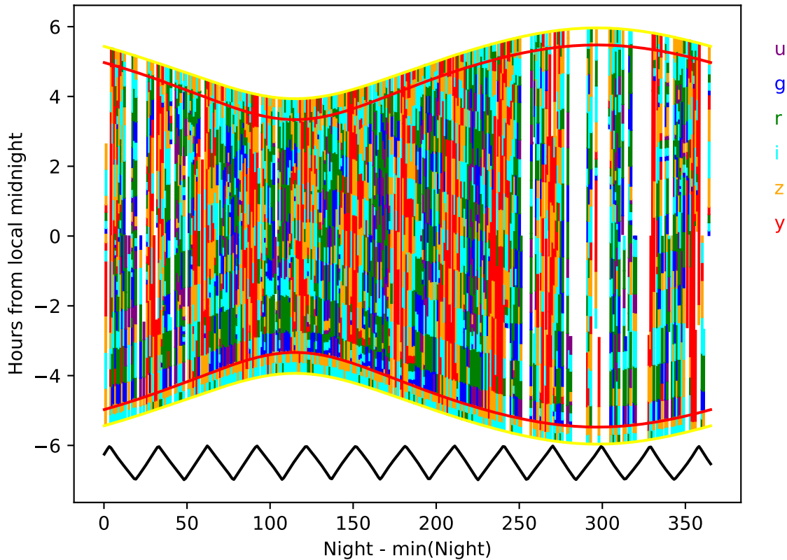
noroll_mjdp120_v3.4_10yrs year 6-7: Hourglass
