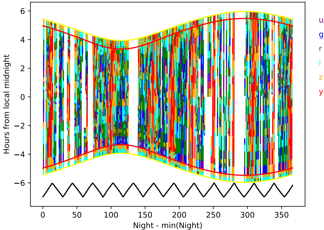
noroll_mjdp120_v3.4_10yrs year 5-6: Hourglass
