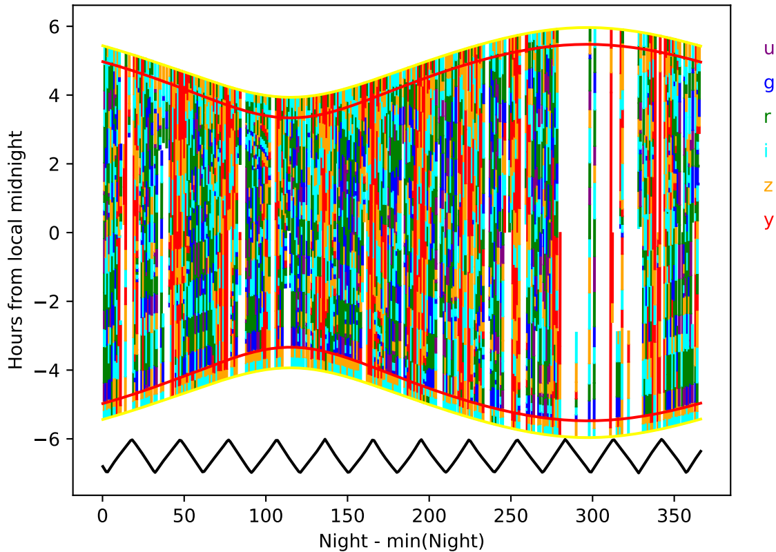
noroll_mjdp120_v3.4_10yrs year 2-3: Hourglass
