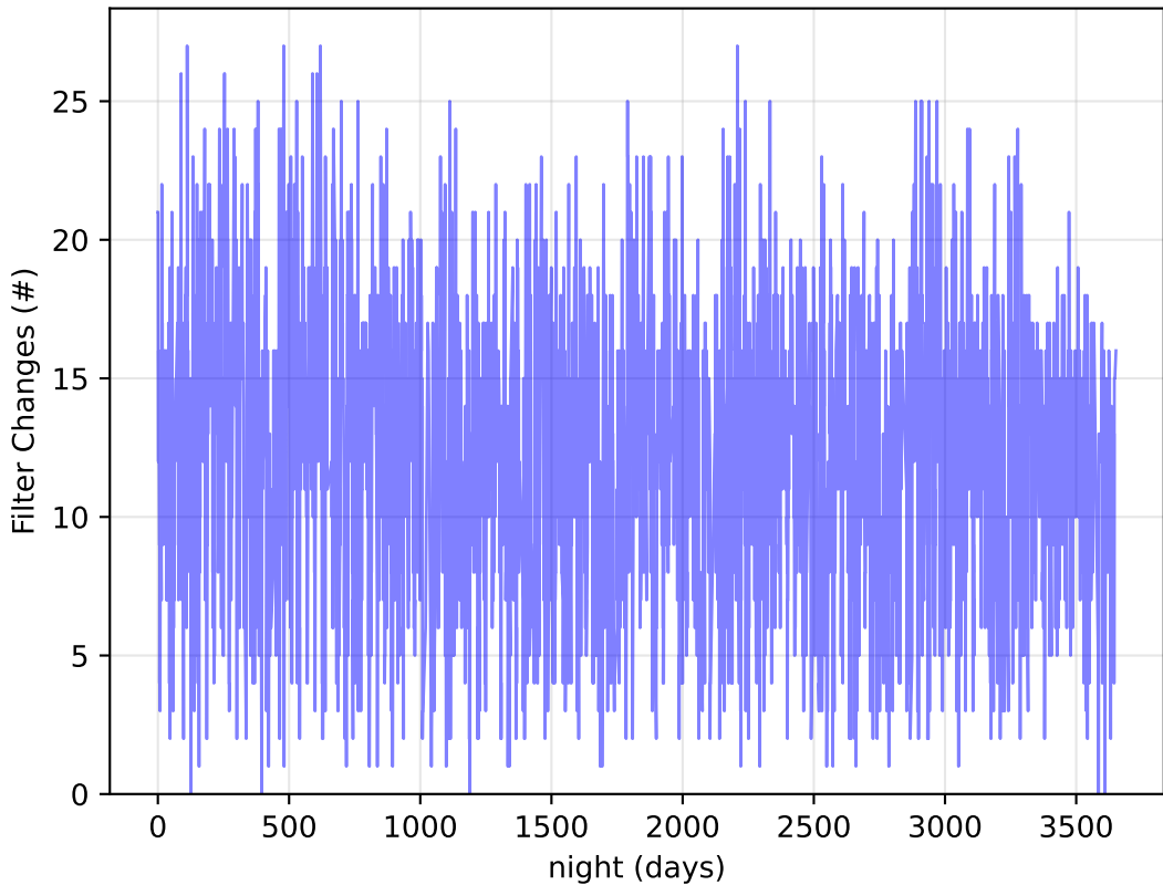
noroll_mjdp120_v3.4_10yrs : Filter Changes
