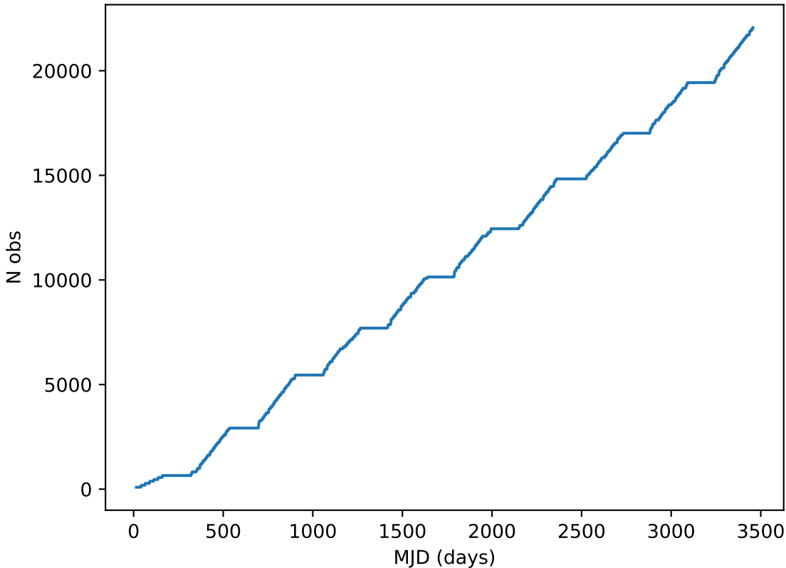
noroll_mjdp120_v3.4_10yrs note like DD:XMM_LSS%: Cumulative
