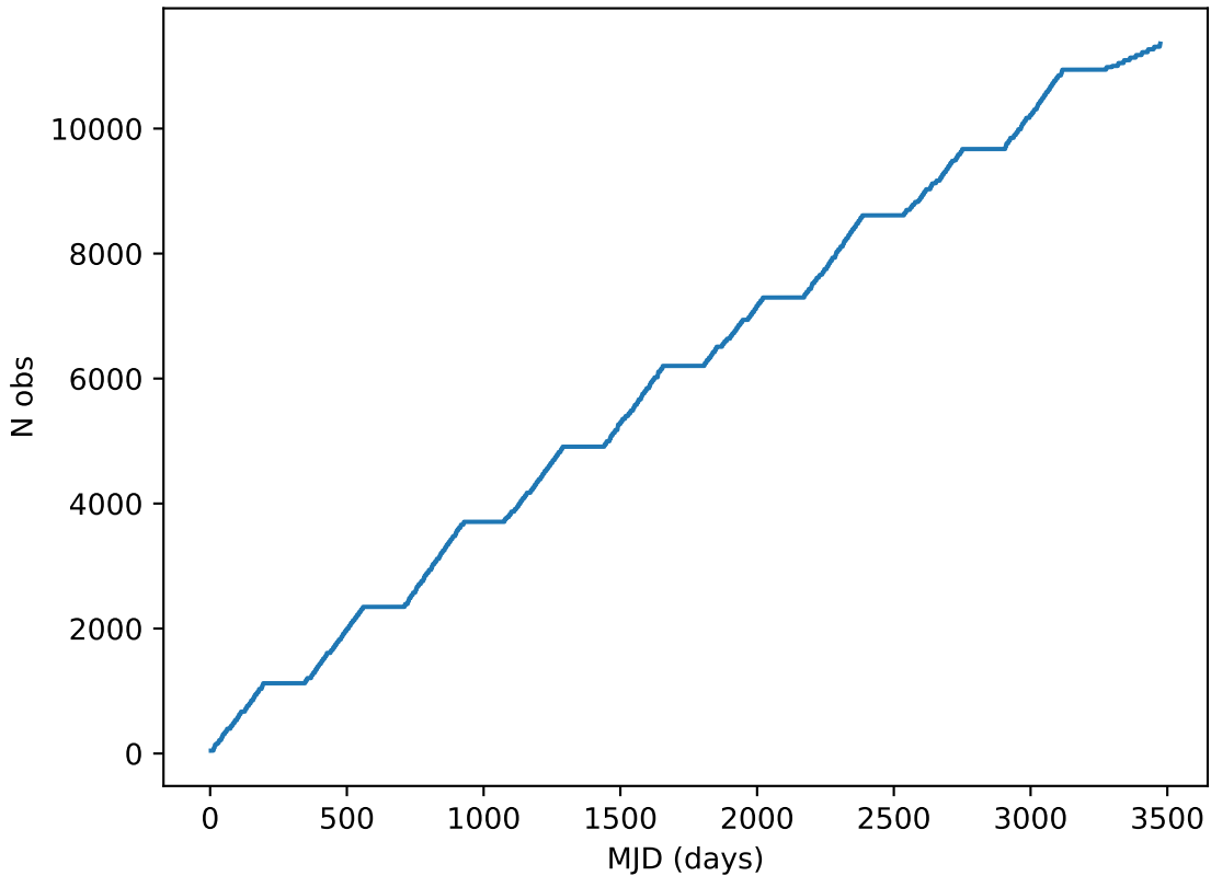
noroll_mjdp120_v3.4_10yrs note like DD:EDFS_b%: Cumulative
