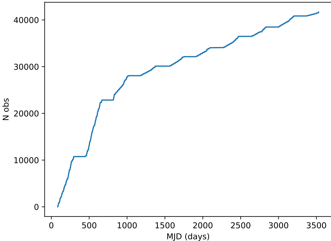
noroll_mjdp120_v3.4_10yrs note like DD:COSMOS%: Cumulative
