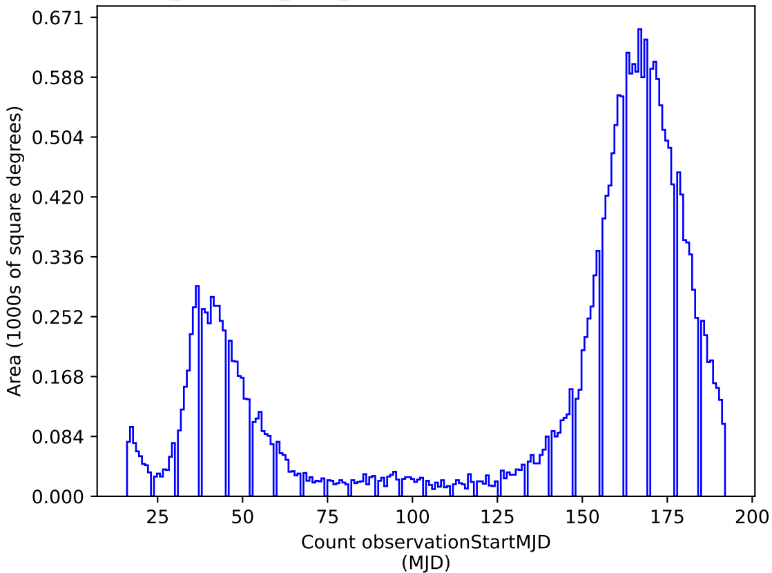
noroll_mjdp120_v3.4_10yrs z: Count observationStartMJD
